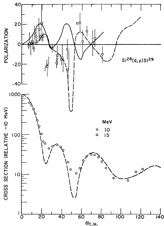
Fig. 2. Polarization of protons from the reaction Si^{28}(d,p)Si^{29}_{g.s.} at E_d=10 and 15 MeV (the latter from Ref. 16). The solid line is the logarithmic derivative of the relative cross section at 10 MeV. The dashed lines are calculated on the basis of the DWBA using spin-orbit terms in both the proton and deuteron potentials. They are taken from Ref. 17.
